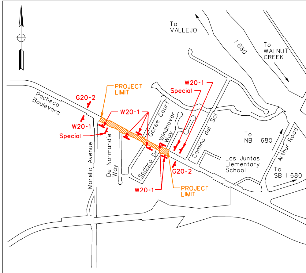
VICINITY AND CONSTRUCTION SIGNING MAP
