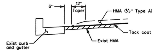
SECTION B-B NO SCALE
