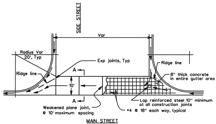
TYPICAL PLAN - VALLEY GUTTER
