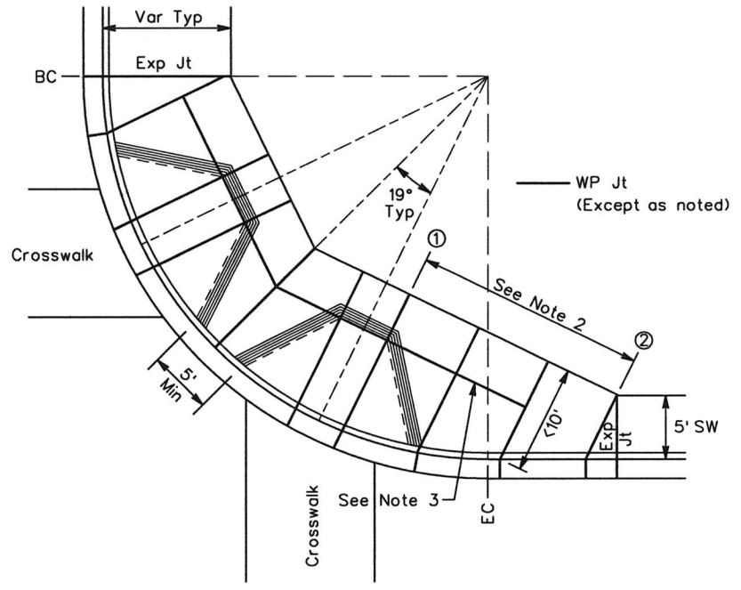
30' RADIUS RETURN
