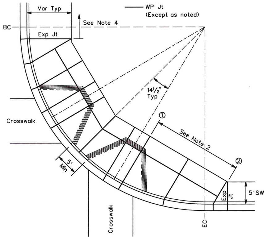
40' RADIUS RETURN
